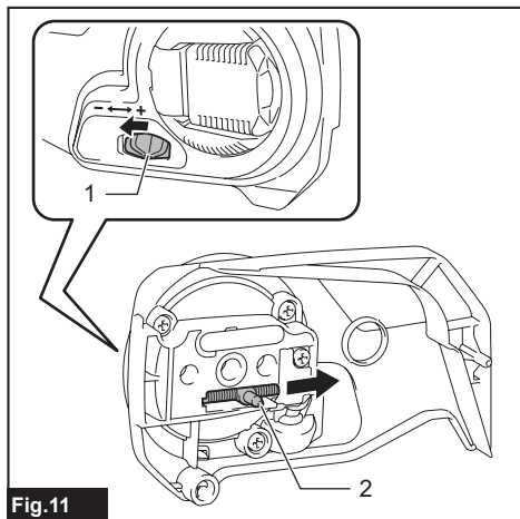
Fig. 11 ► 1. Adjusting dial 2. Adjusting pin
